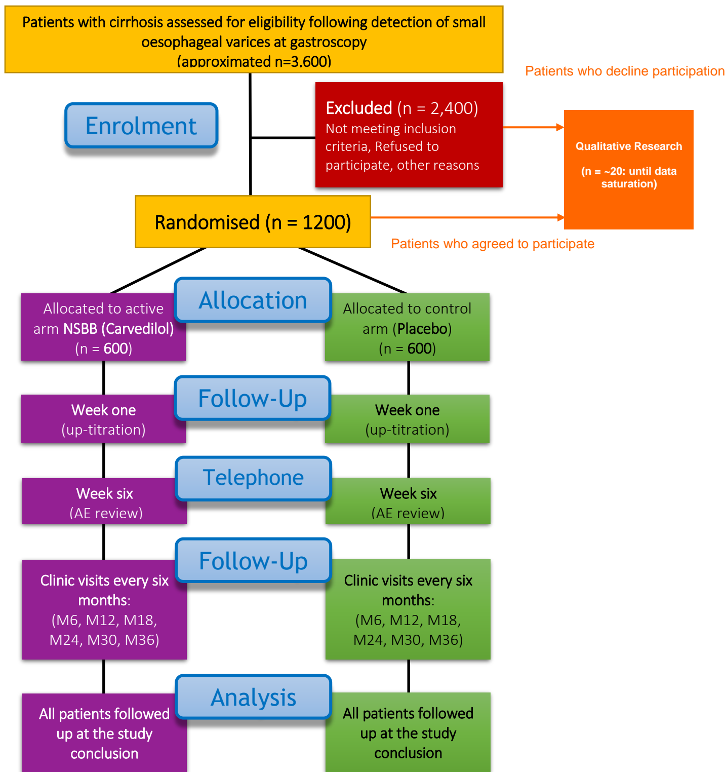
Figure 2: Trial flowchart
